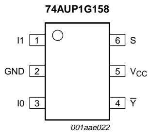
Fig 5. Pin configuration SOT363 (SC-88)
